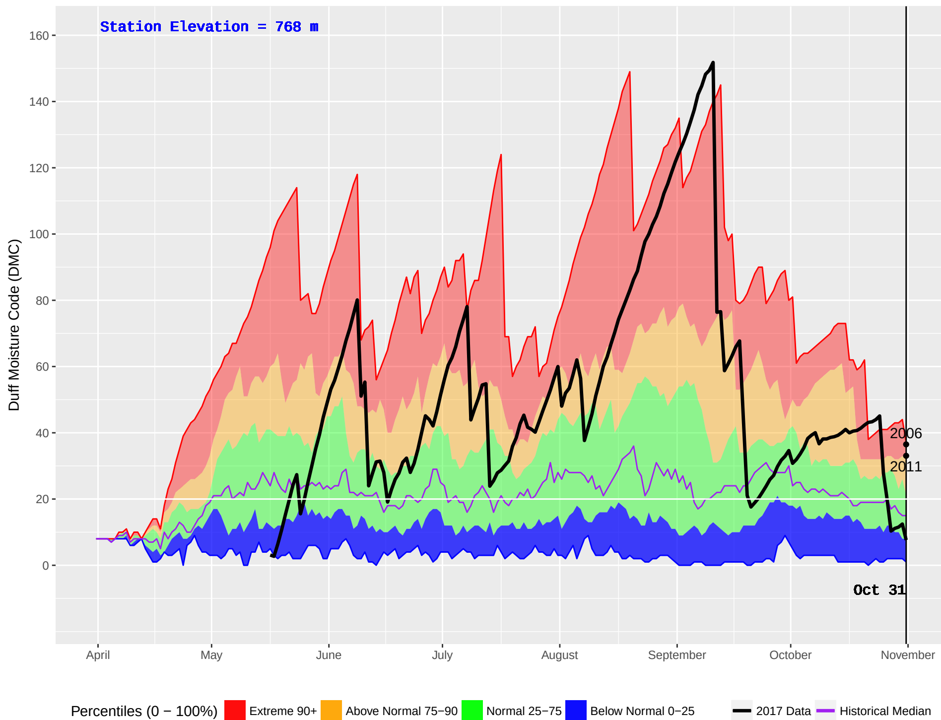
GRAHAM (124) : Historical (1979–2016) and Current (2017) Noon Duff Moisture Code (DMC)
