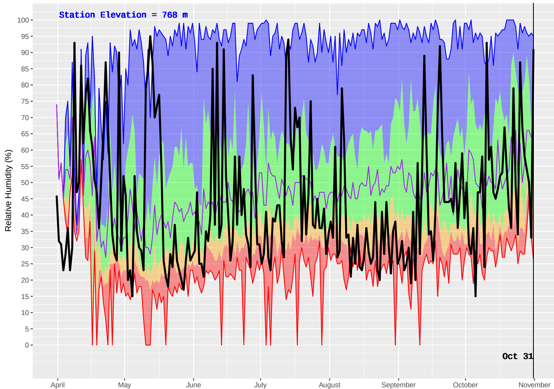
GRAHAM (124) : Historical (1979–2016) and Current (2017) Noon Relative Humidity
