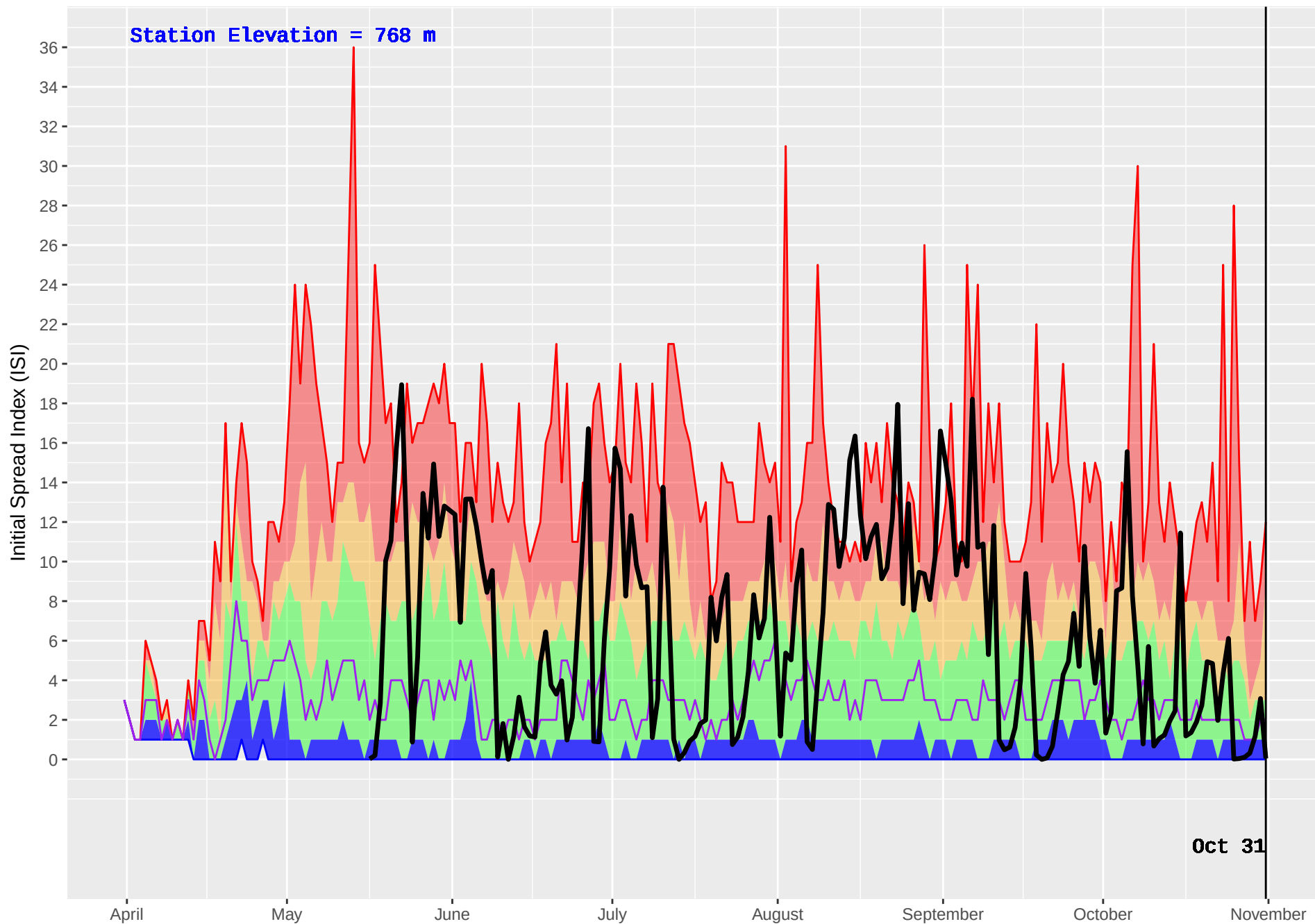
GRAHAM (124) : Historical (1979–2016) and Current (2017) Noon Initial Spread Index (ISI)
