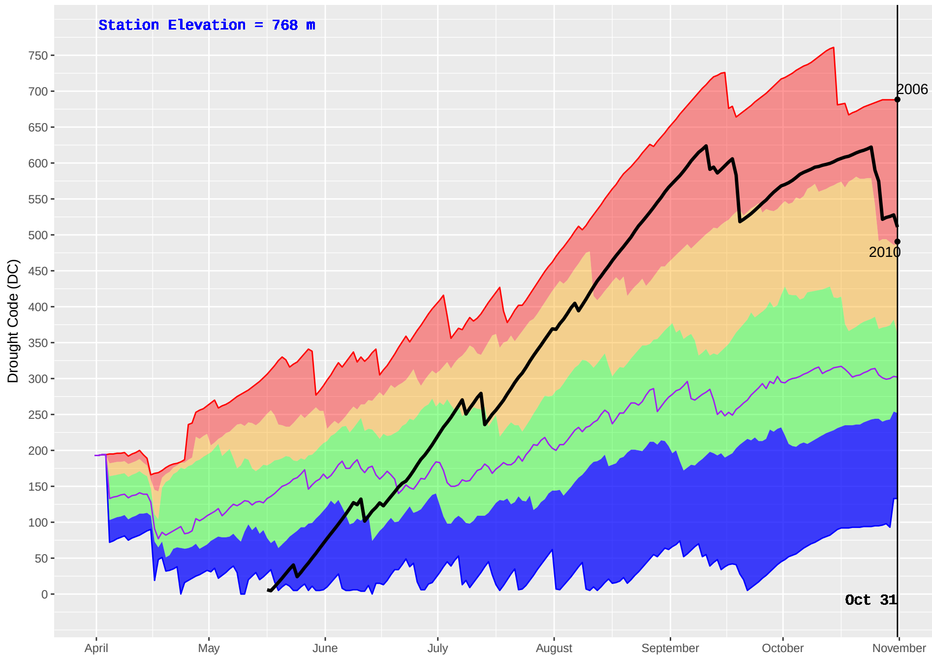
GRAHAM (124) : Historical (1979–2016) and Current (2017) Noon Drought Code (DC)
