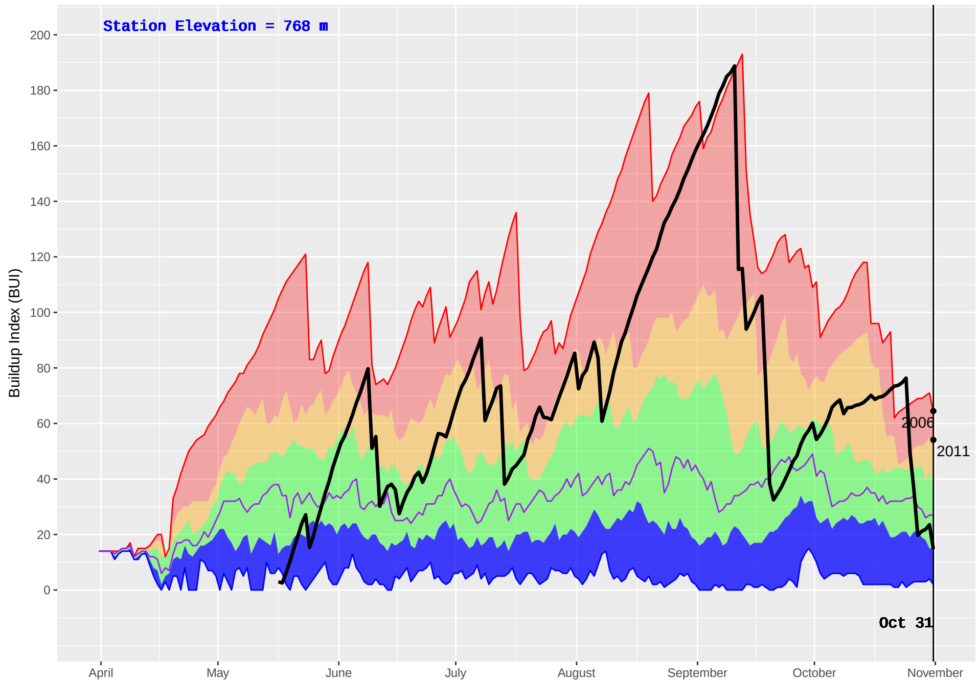
GRAHAM (124) : Historical (1979–2016) and Current (2017) Noon Buildup Index (BUI)
